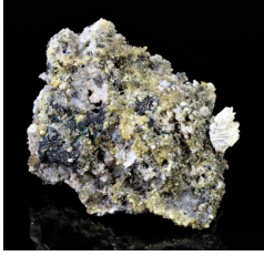
Cerussite/Mimetite - Tsumeb
